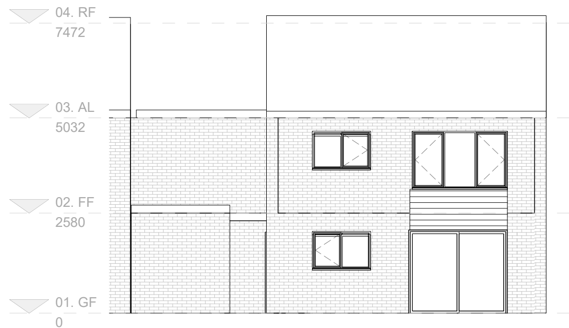
02. Rear Elevation Existing 1 : 100
