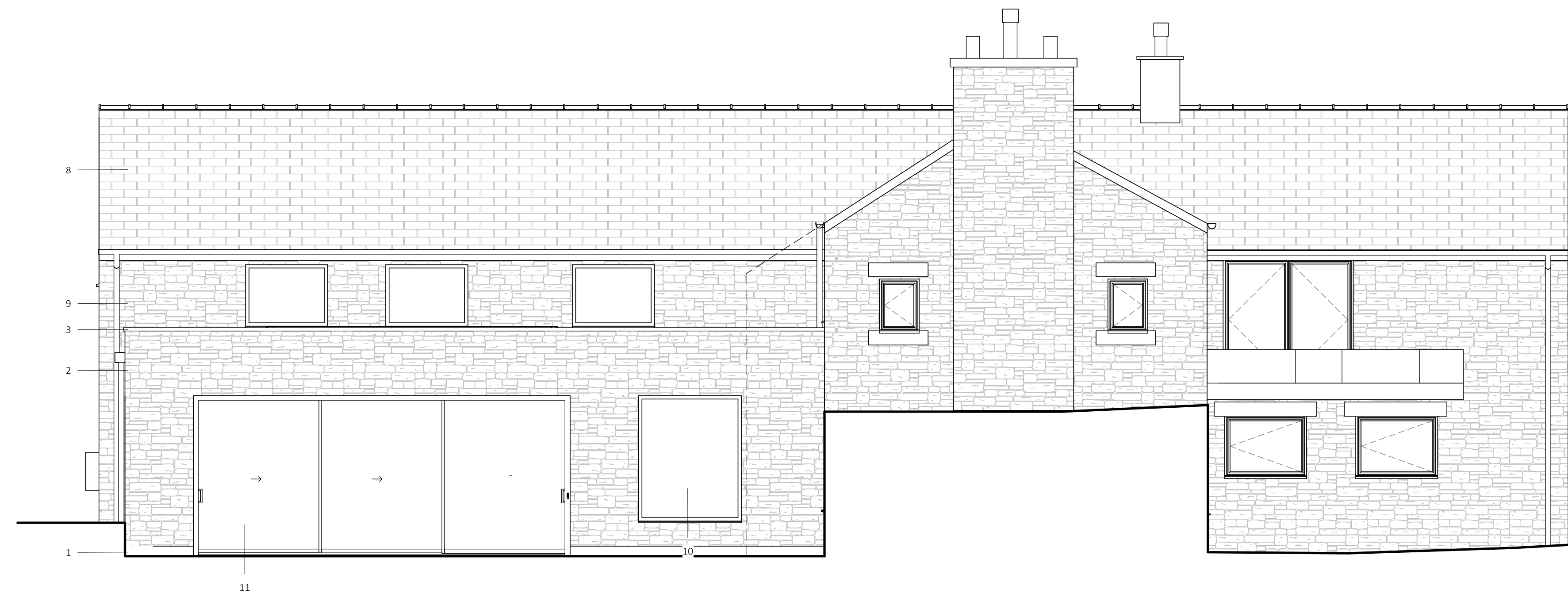
1 Proposed North Elevation 1 : 50
