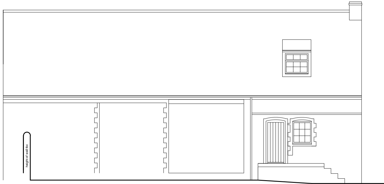
Outbuilding (South-West) - AS EXISTING
