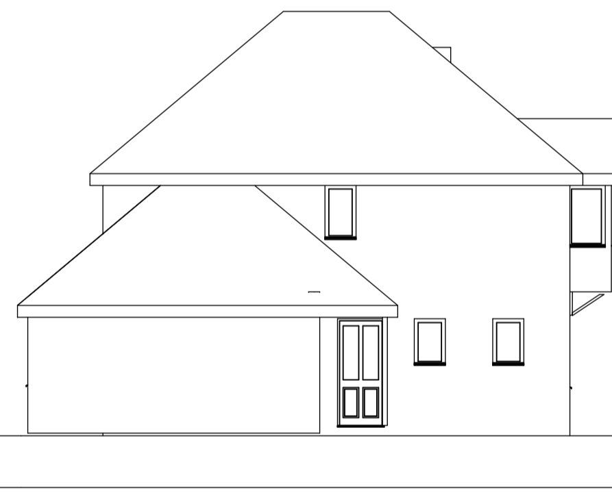
6 Existing North Elevation 1:100
