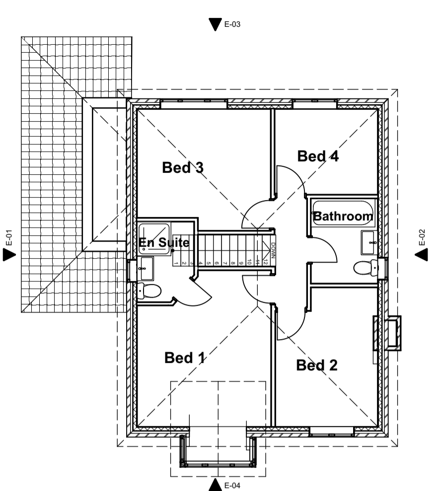
5 Proposed First Floor 1:100
