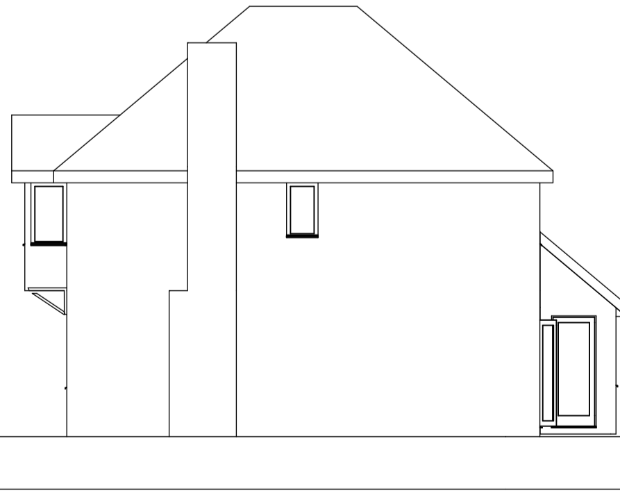
11 Proposed South Elevation 1:100
