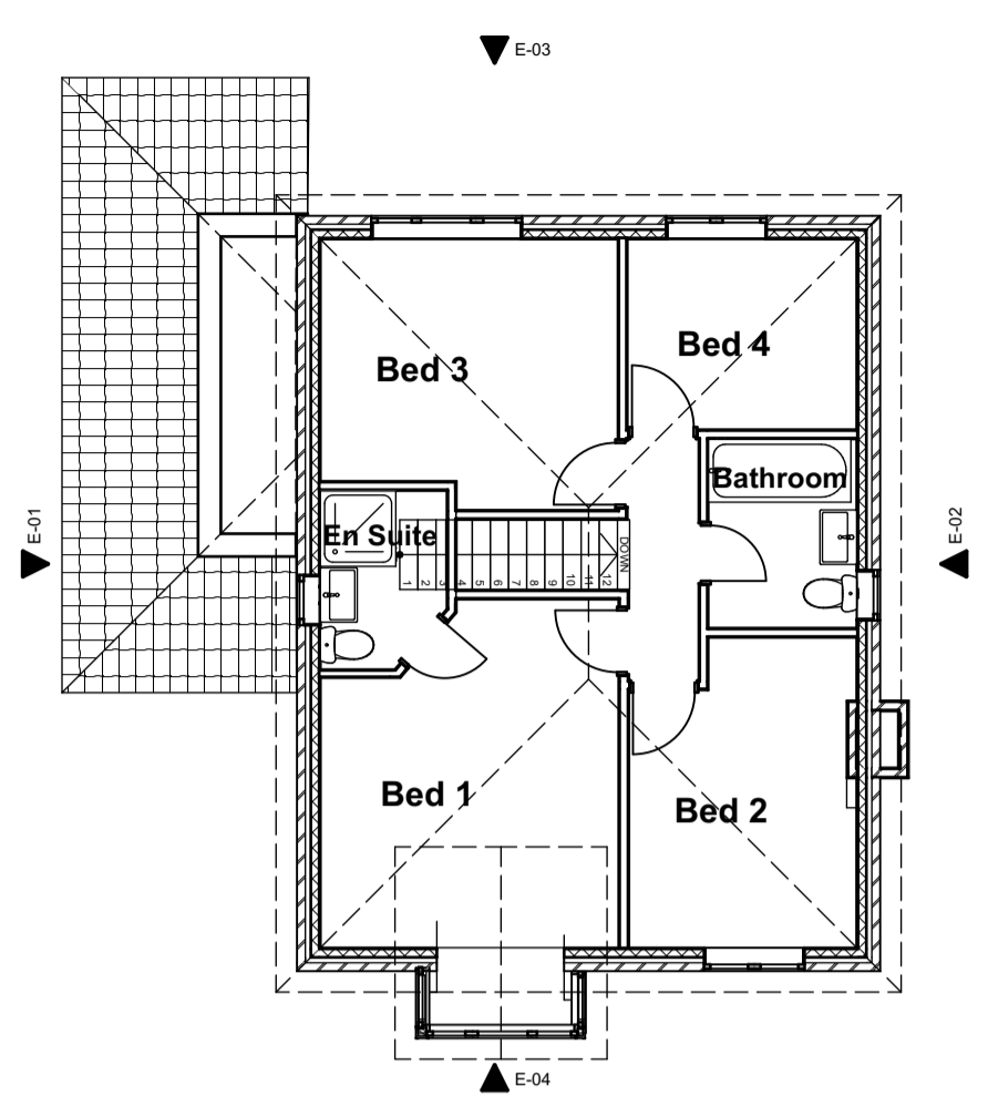
3 Existing First Floor 1:100
