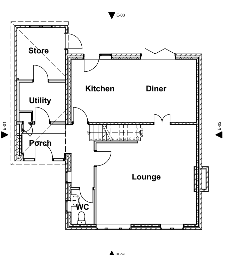
4 Proposed Ground Floor 1:100
