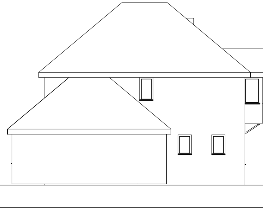
10 Proposed North Elevation 1:100
