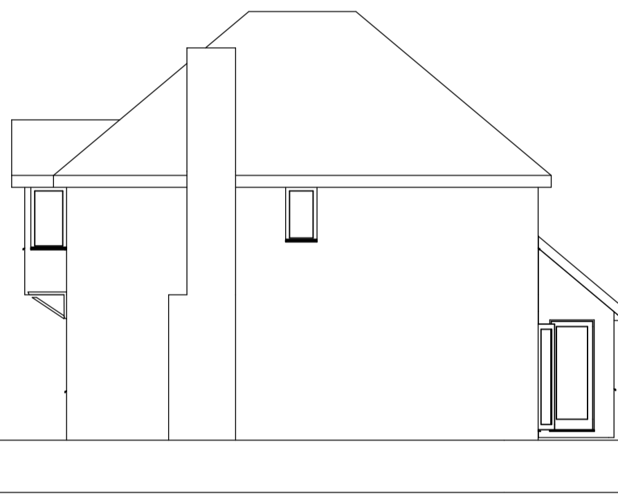
7 Existing South Elevation 1:100
