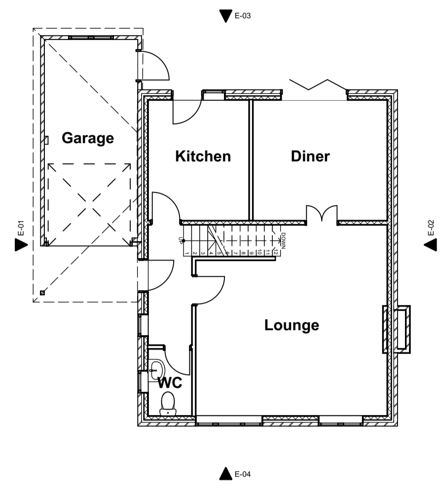
2 Existing Ground Floor 1:100
