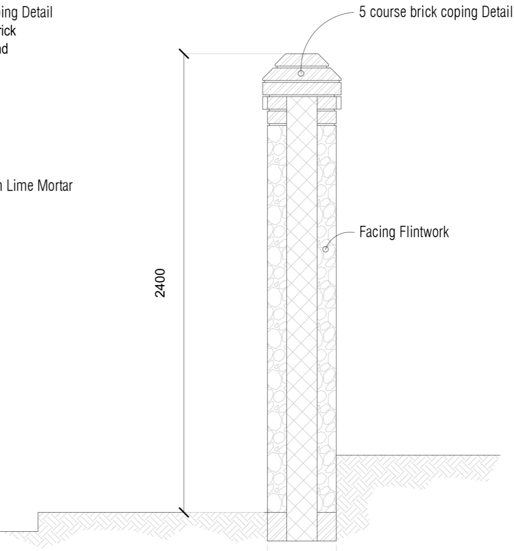
Proposed Wall Cross Section
