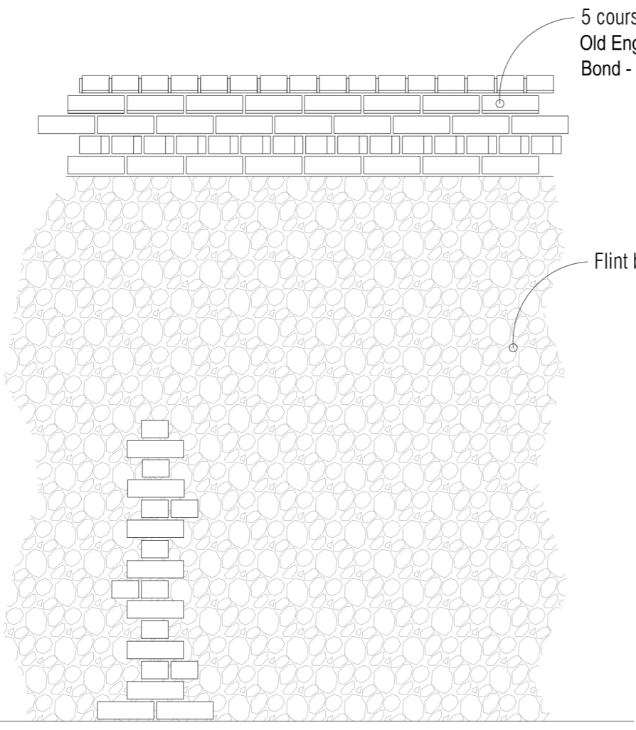
Typical Elevation of new wall
