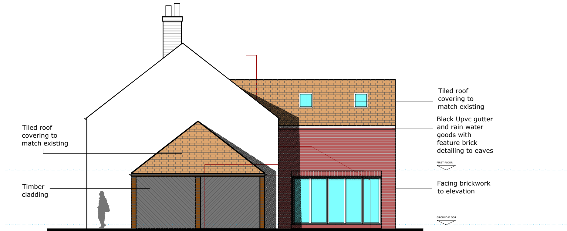
West Elevation
