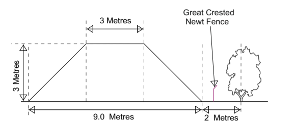
Inset 1 Typical Cross Section through bund
