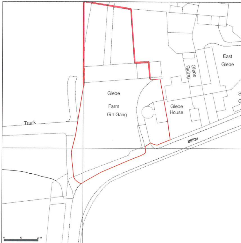
The Gin Gang, Whalton, Morpeth, NE61 3YH. Location Plan: 2Ha @ scale 1:1250 on A4 sheet.
