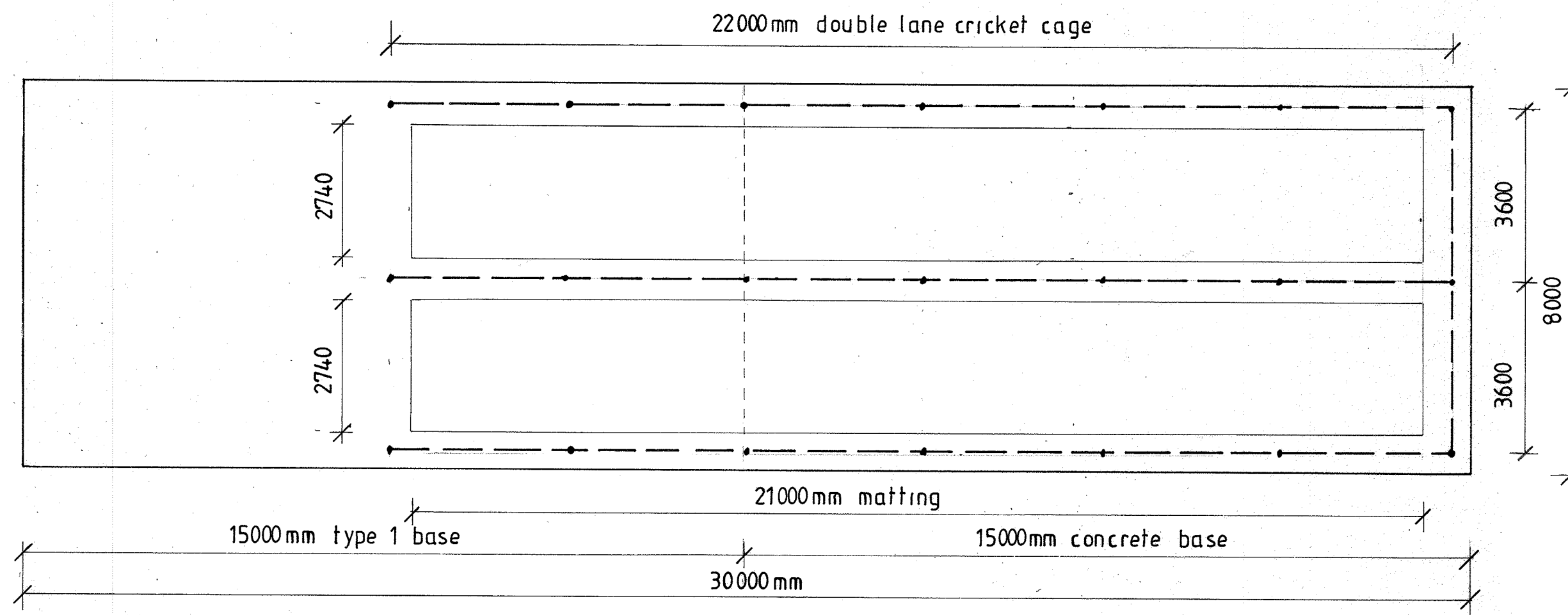
PLAN
