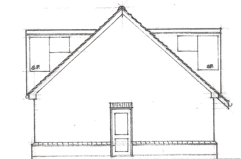
LHSIDE 1:100
