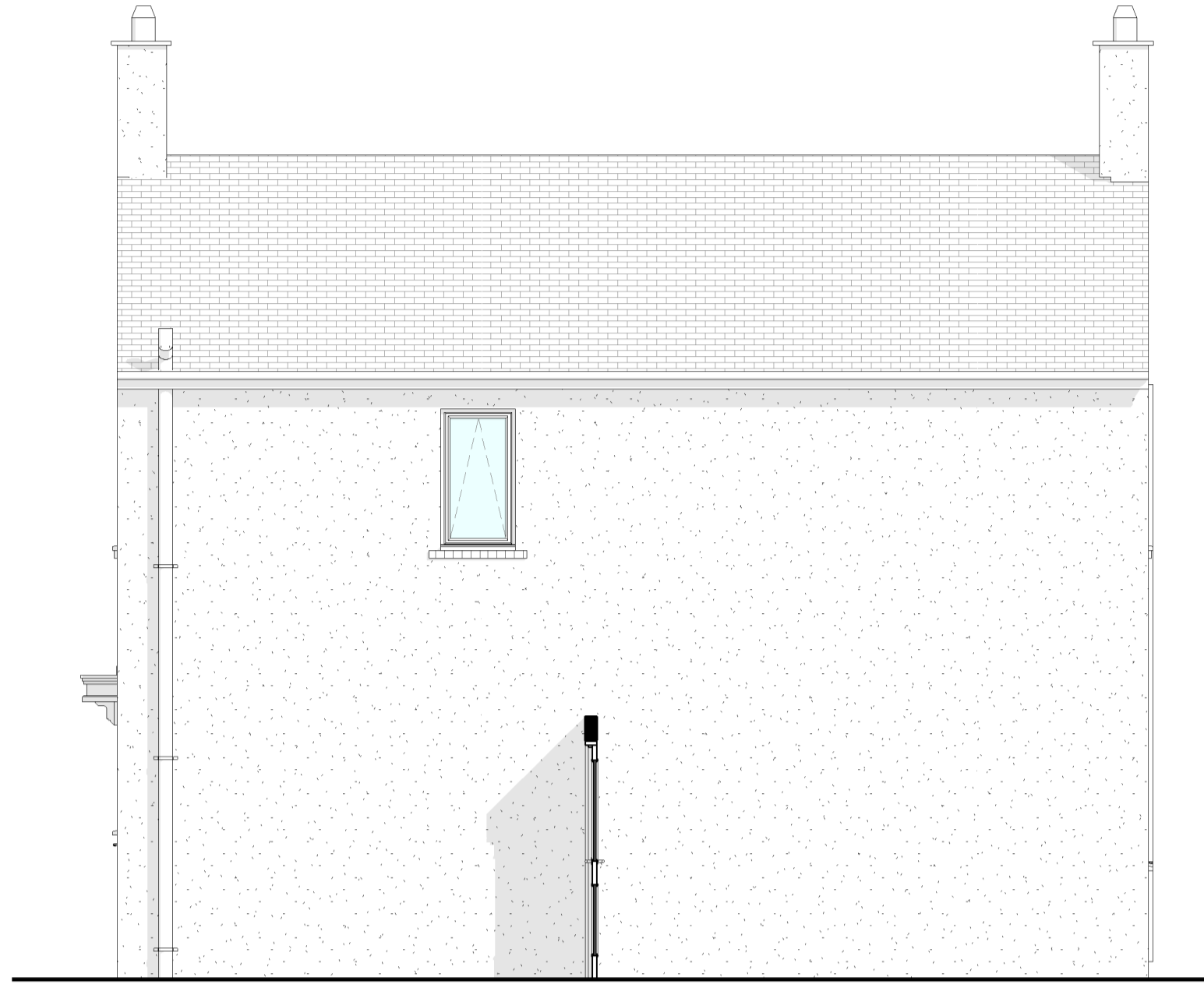
0.1 Proposed Rear Elevation.
