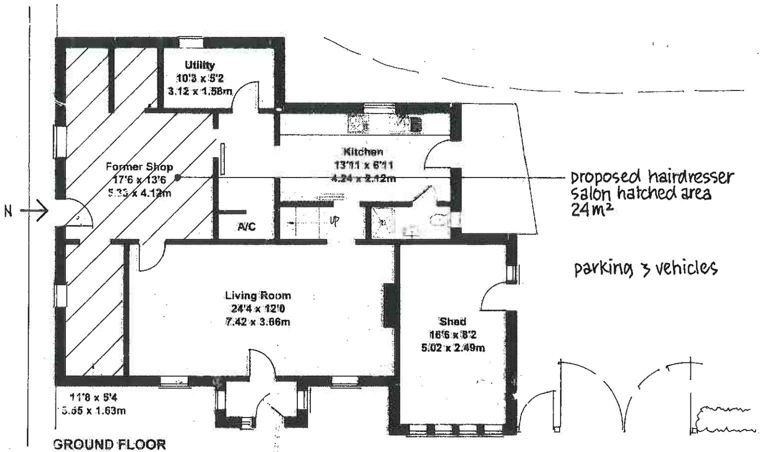
FLOOR PLAN 1:100 @ A4
