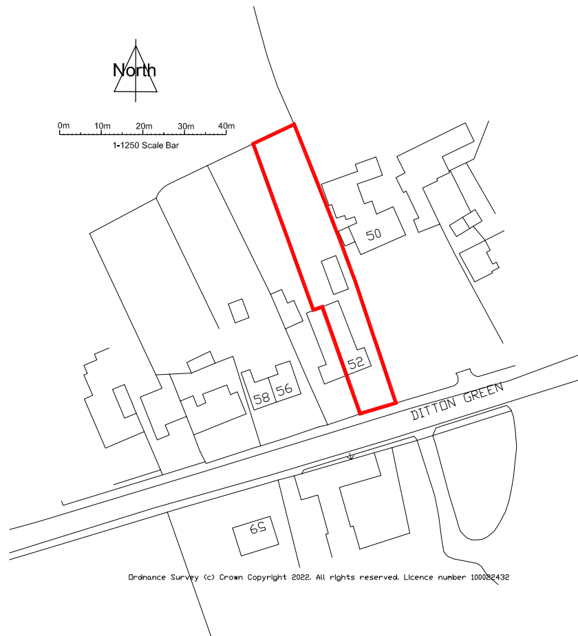
Site Location Plan Scale 1-1250@A4
