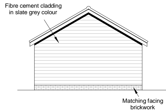
PROPOSED SIDE(E) ELEVATION 1:100
