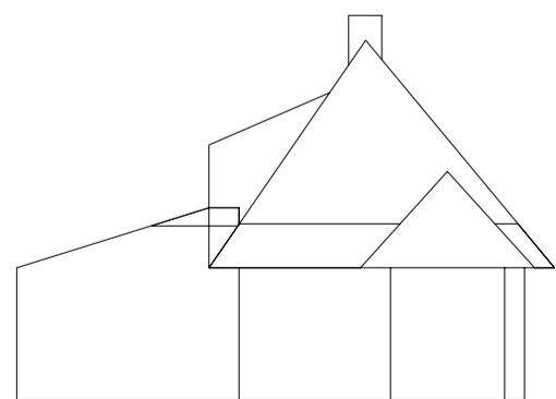
Left elevation
