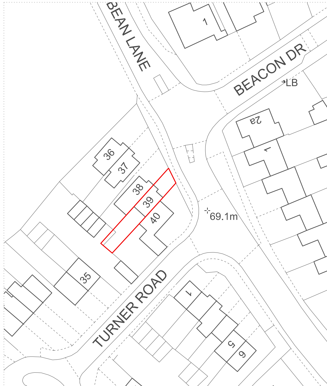
BLOCK PLAN - EXISTING SCALE 1:500 @ A3
