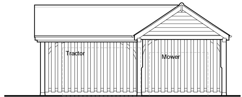
North Elevation 1:100
