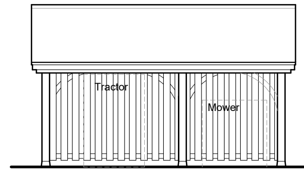
West Elevation 1:100
