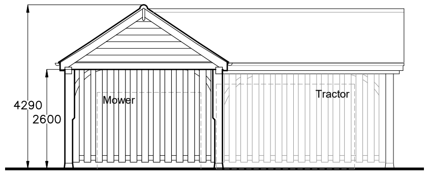
South Elevation 1:100
