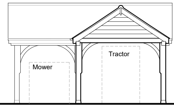
East Elevation 1:100
