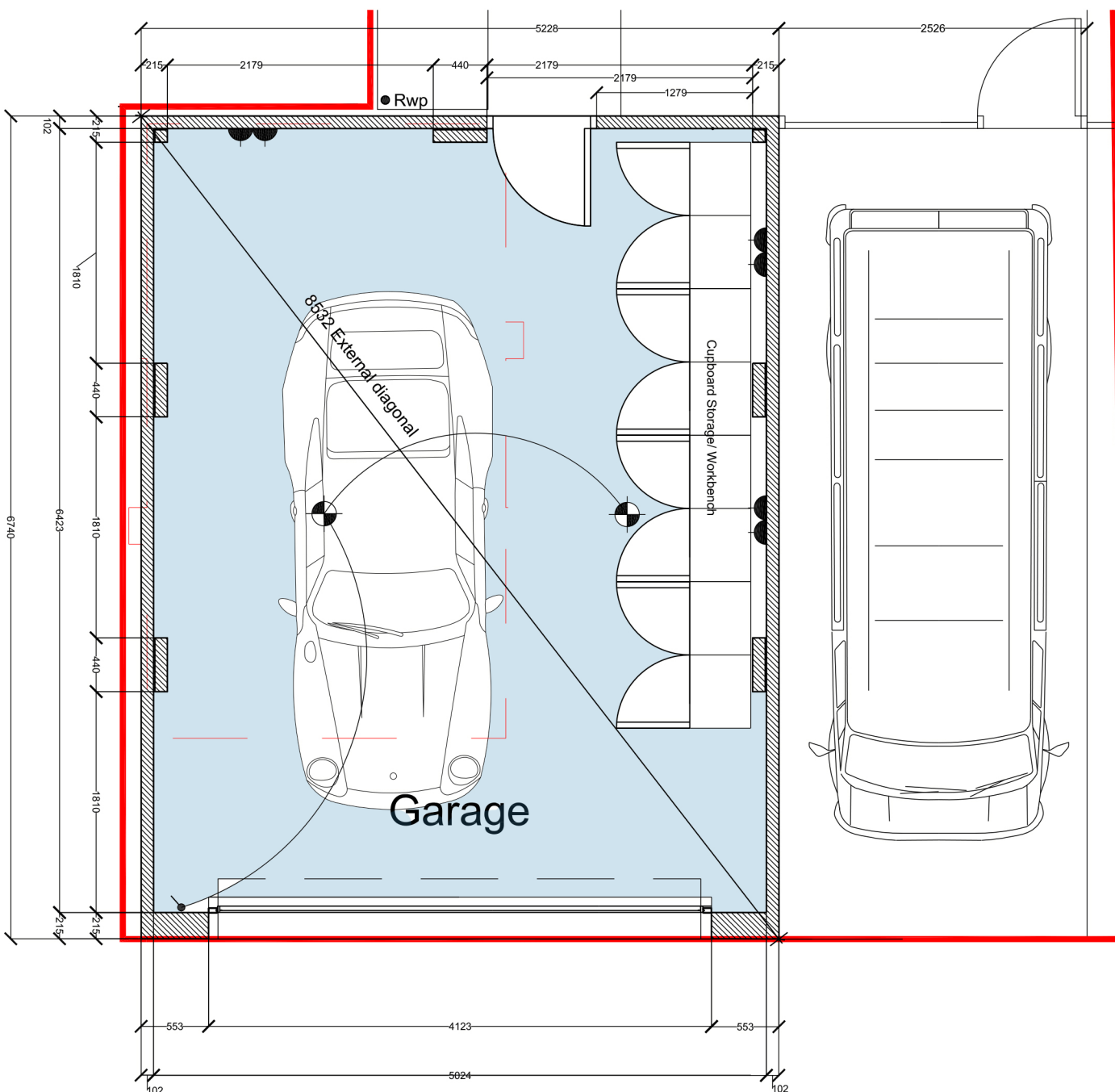
Proposed Garage Plan 1:50
