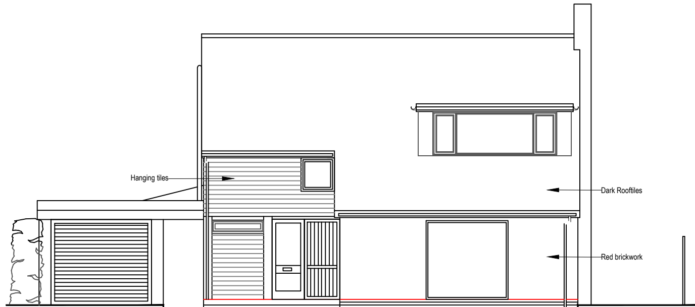
North elevation 1:100
