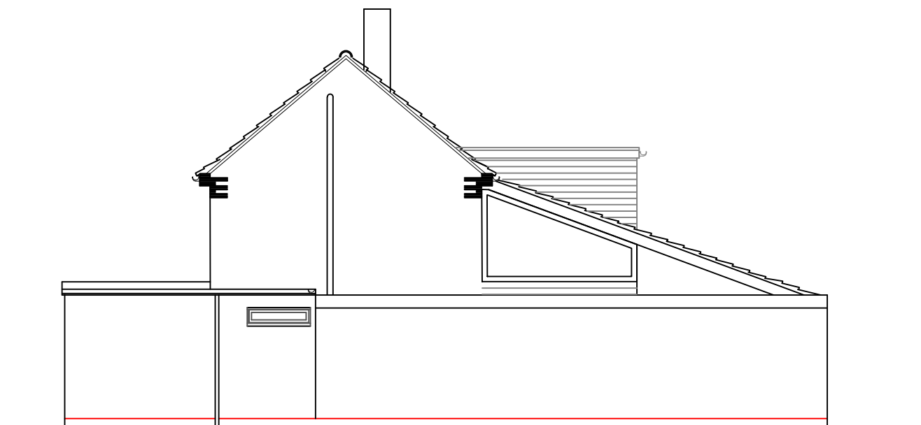
East Elevation 1:100
