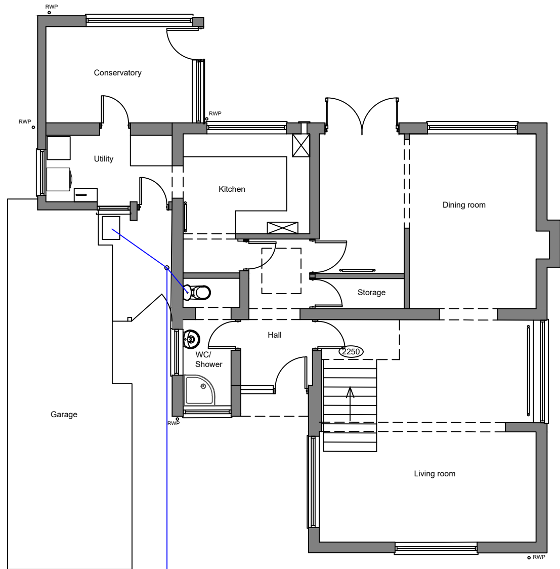
Ground floor 1:100
