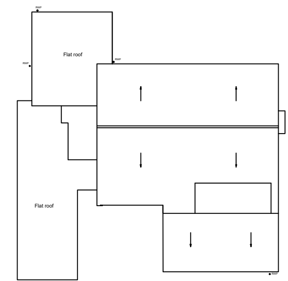
Roof plan 1:200
