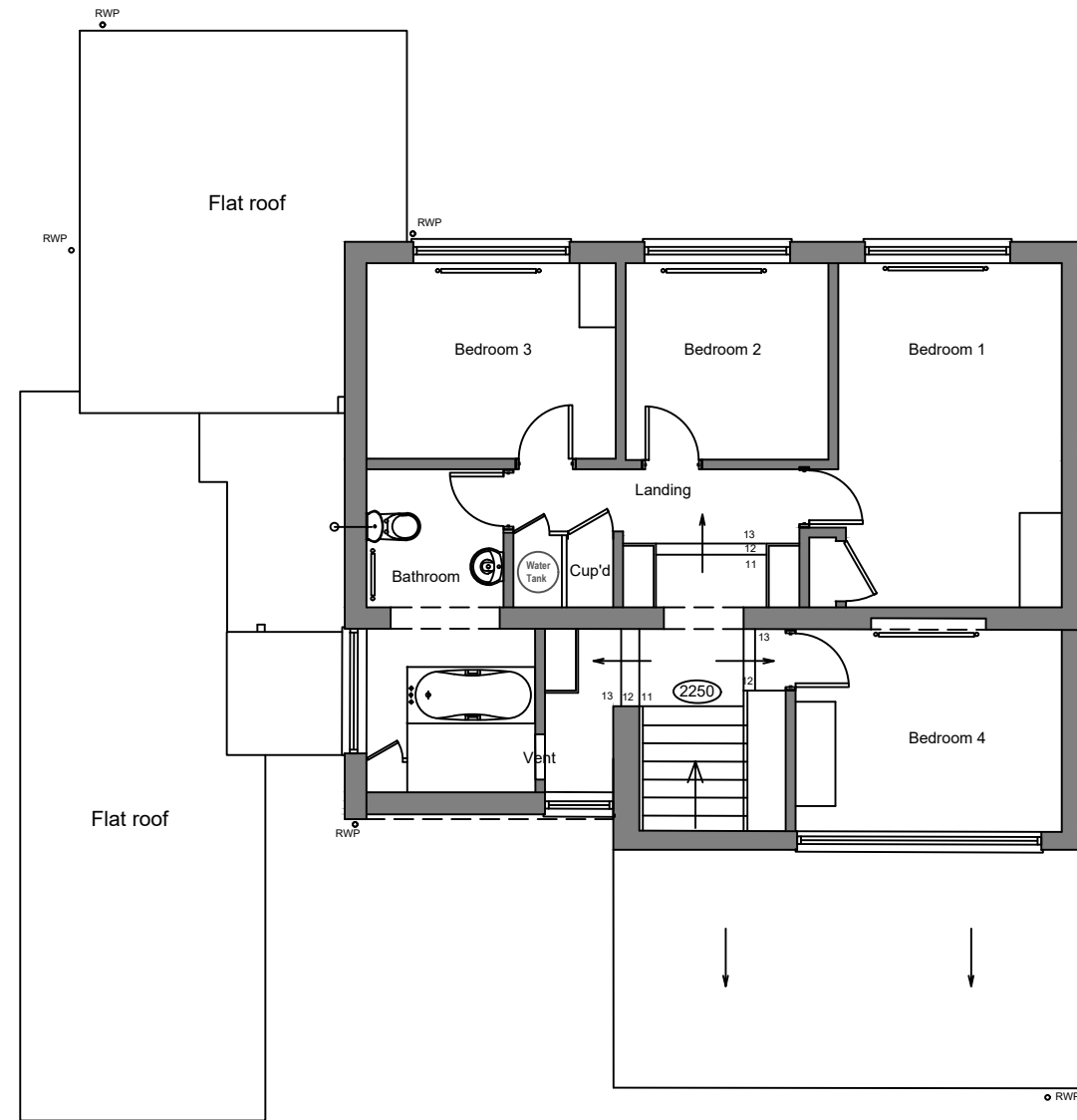
First floor 1:100
