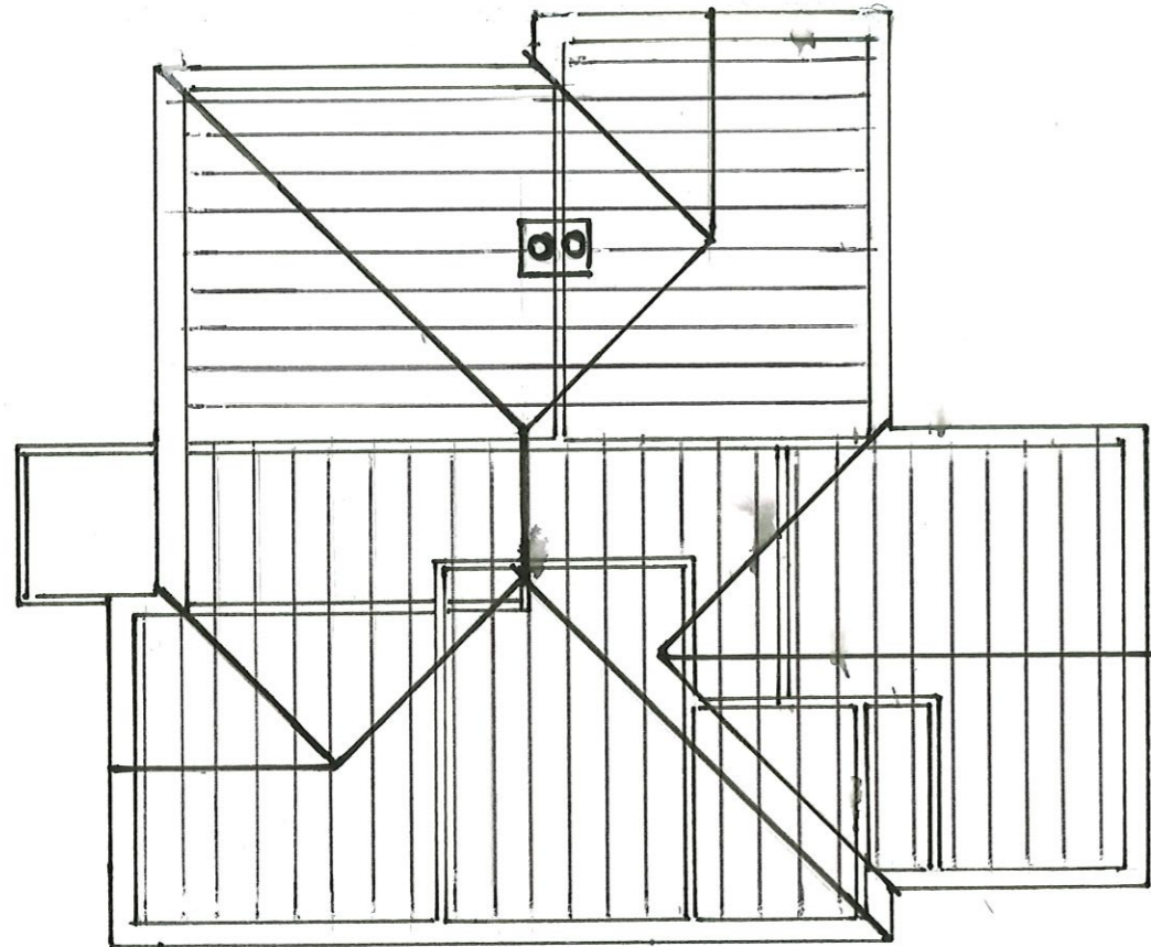
Roof layout
