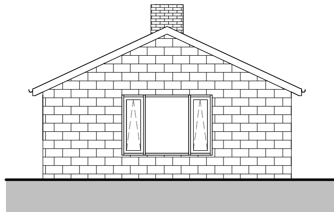
South East Elevation as Existing 1 : 100
