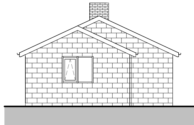
North West Elevation as Existing 1 : 100
