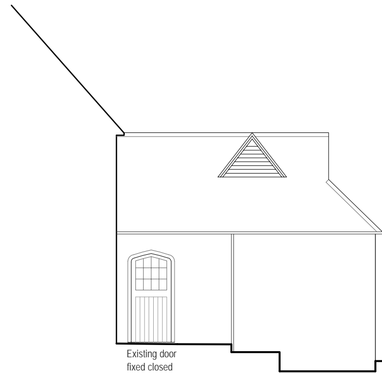
SOUTH-EAST INTERNAL ELEVATION as proposed
