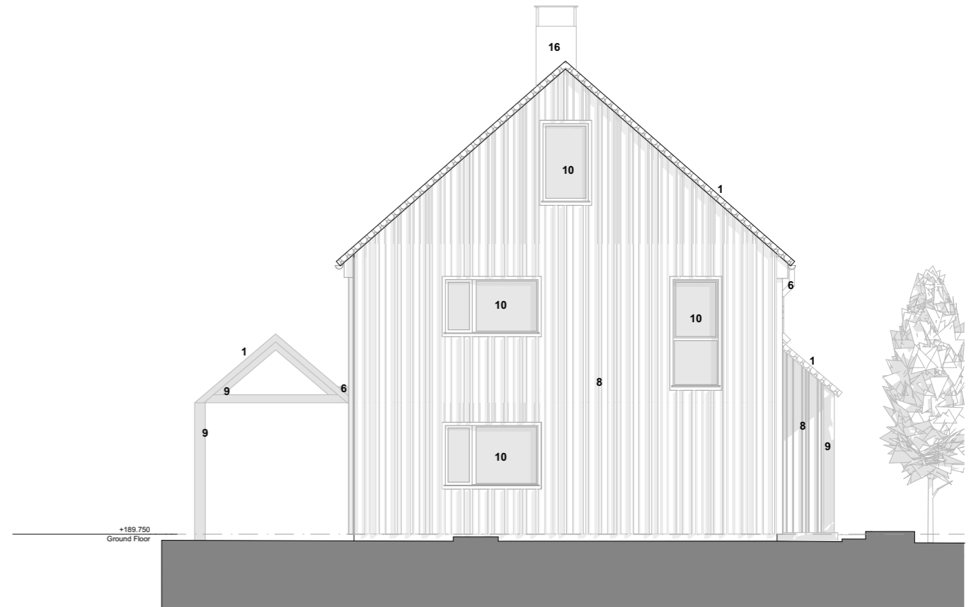
2 SOUTH ELEVATION 1:100
