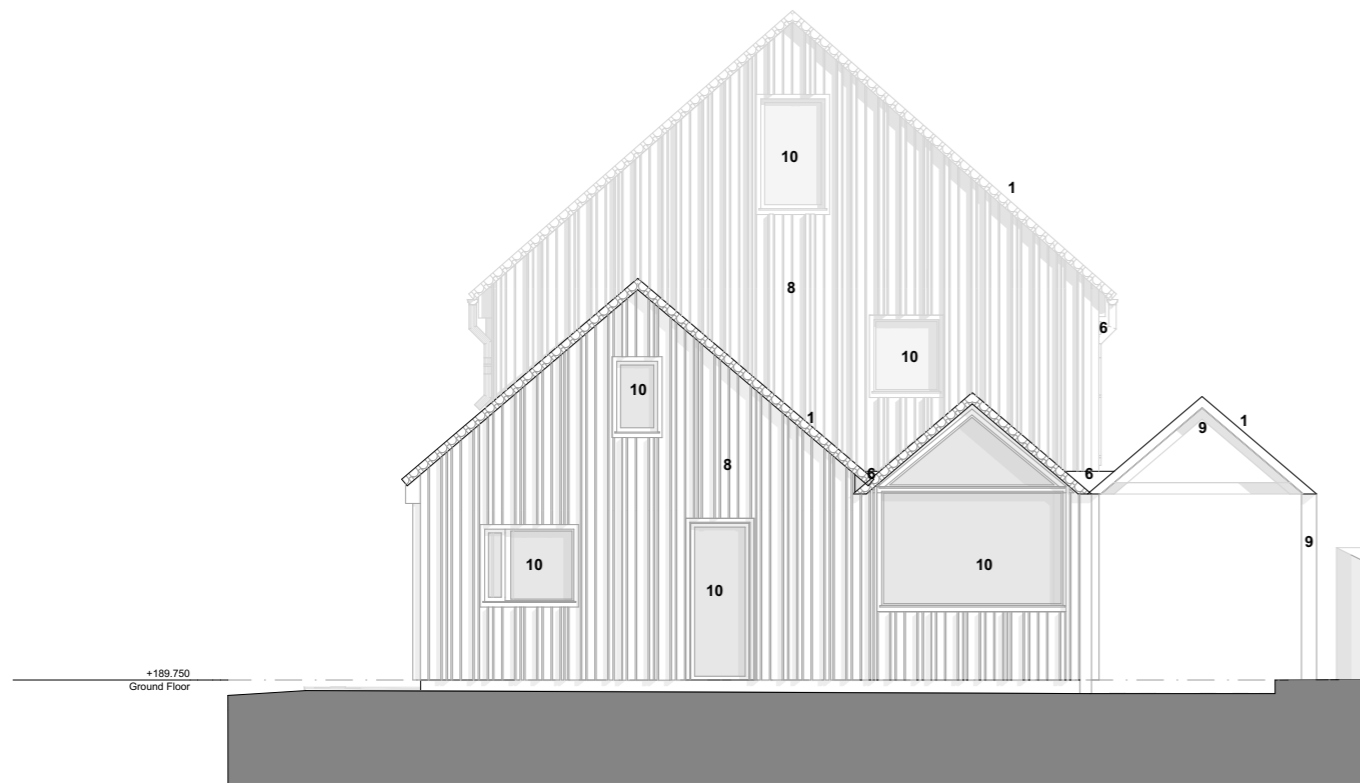
1 NORTH ELEVATION 1:100
