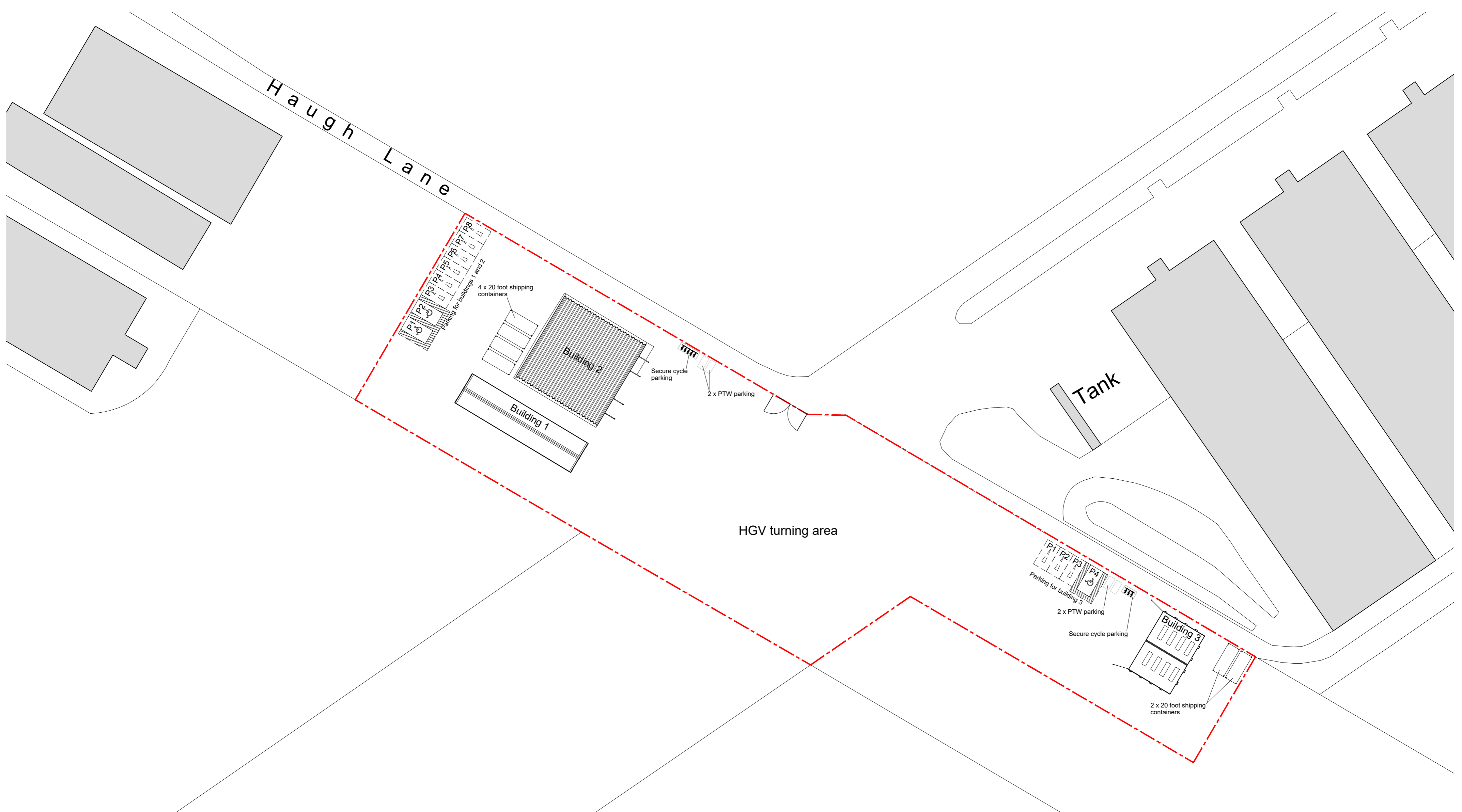
Proposed Site Layout Plan (1:500)
