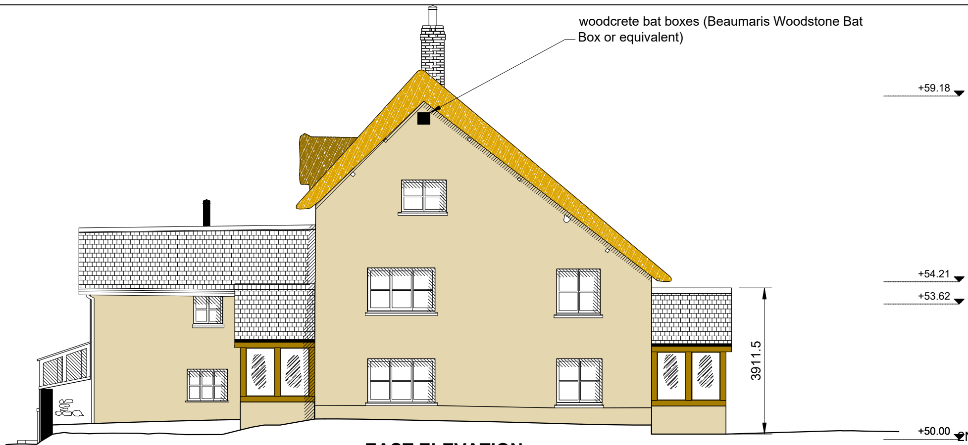
EAST ELEVATION
