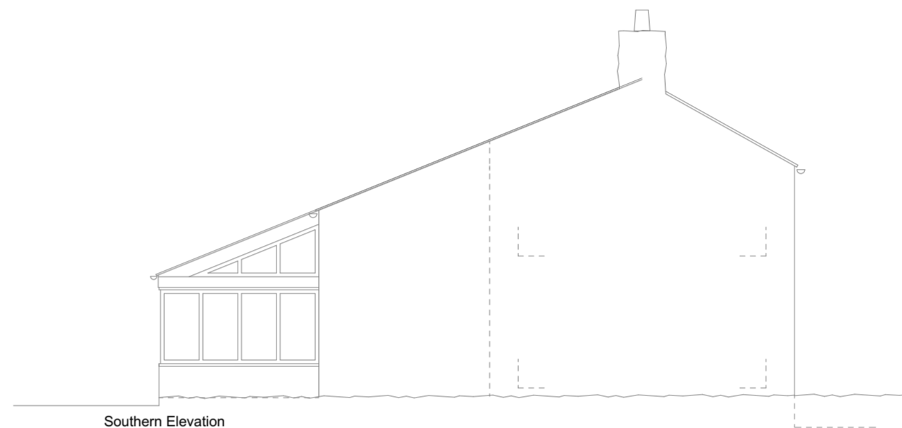
Southern Elevation
