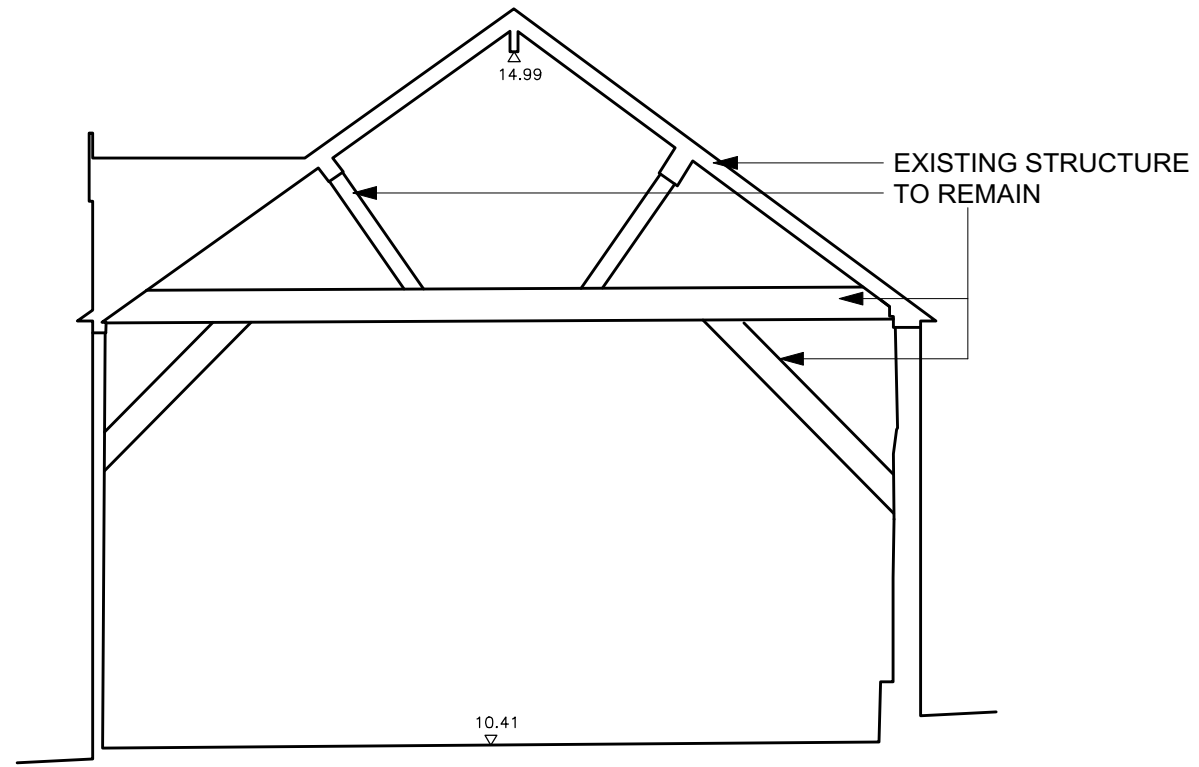
SECTION 1
