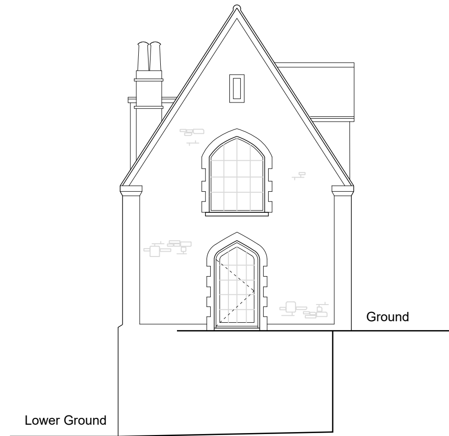
South elevation
