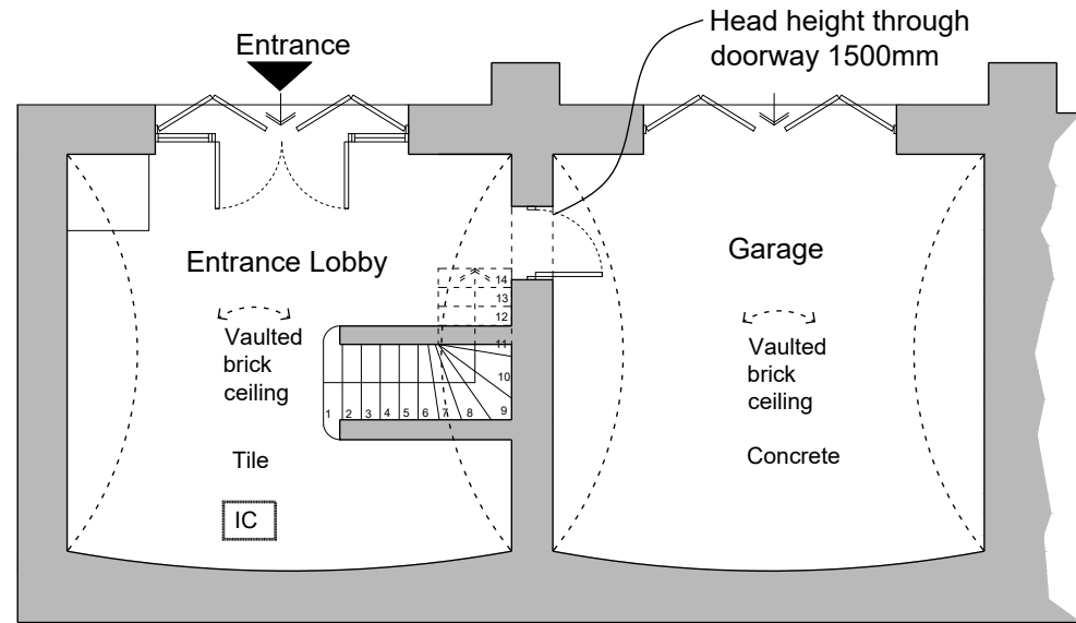
Lower Ground Floor Plan
