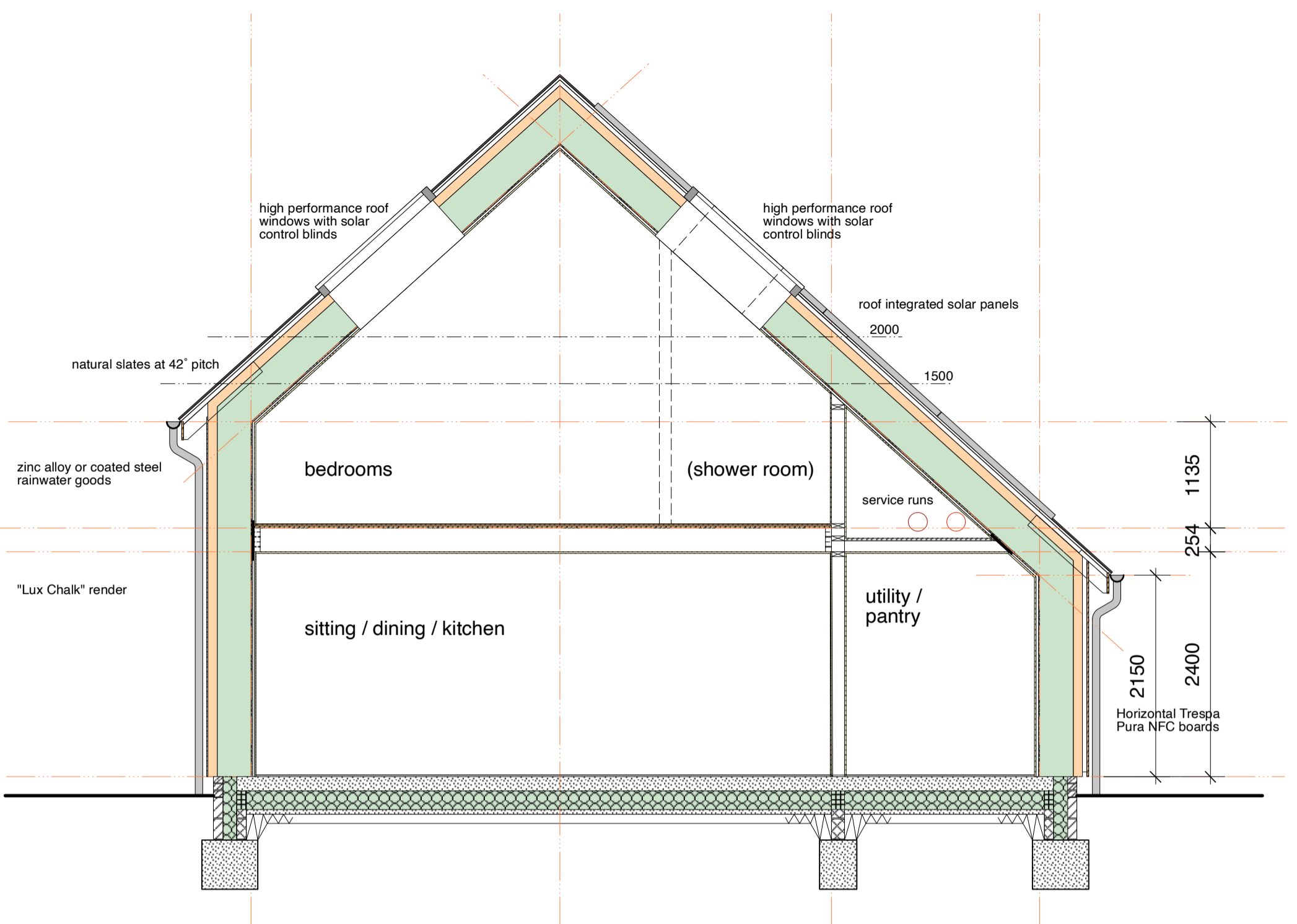
SECTION THROUGH MAIN HOUSE
