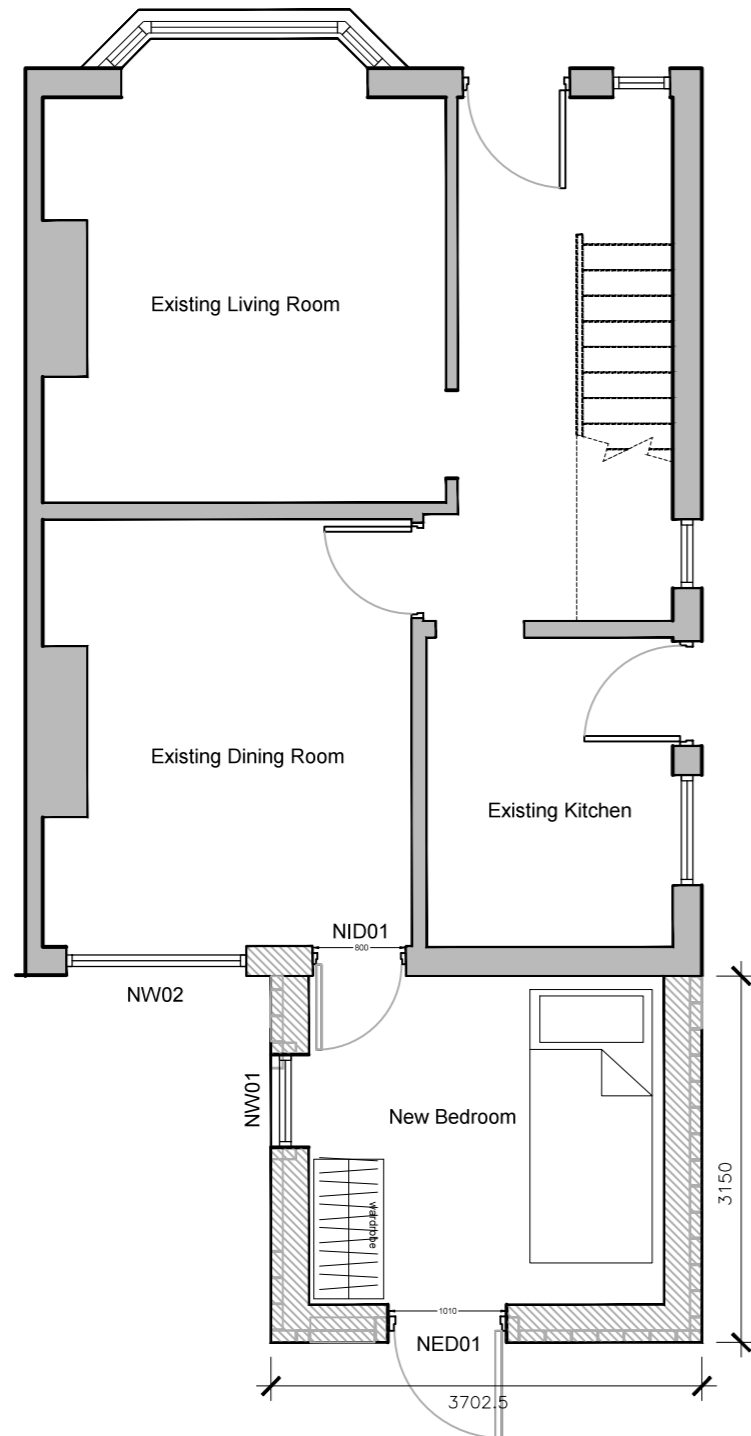
01 | PROPOSED GROUND FLOOR PLAN 1:65 @ A3
