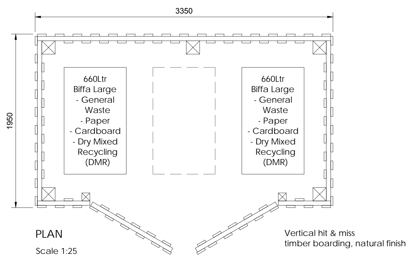
Typical detail for 2.1m high timber hit & miss fence to Bin Enclosure
