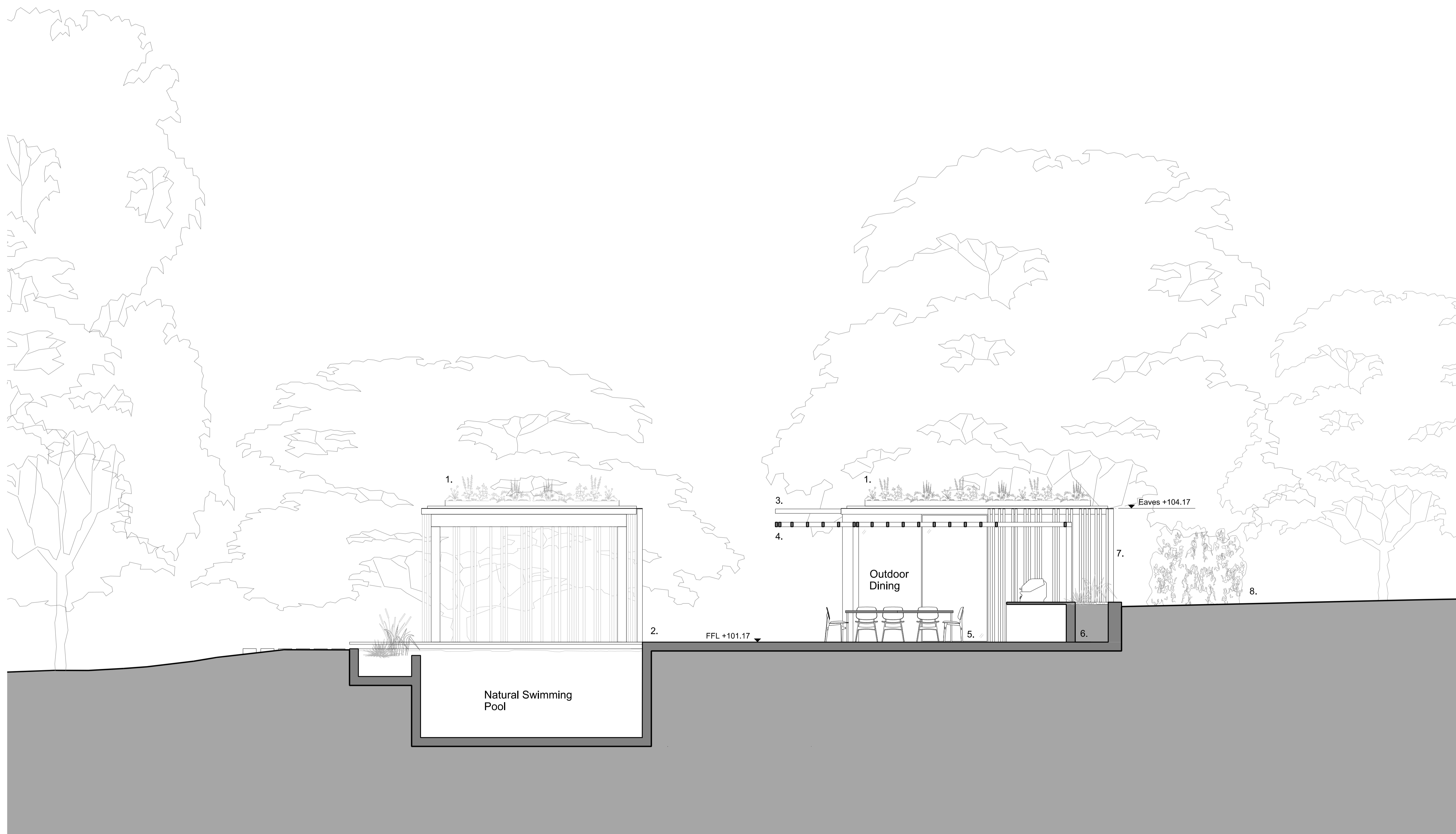
01 Proposed Pool House: Section CC 1:50 @ A1
