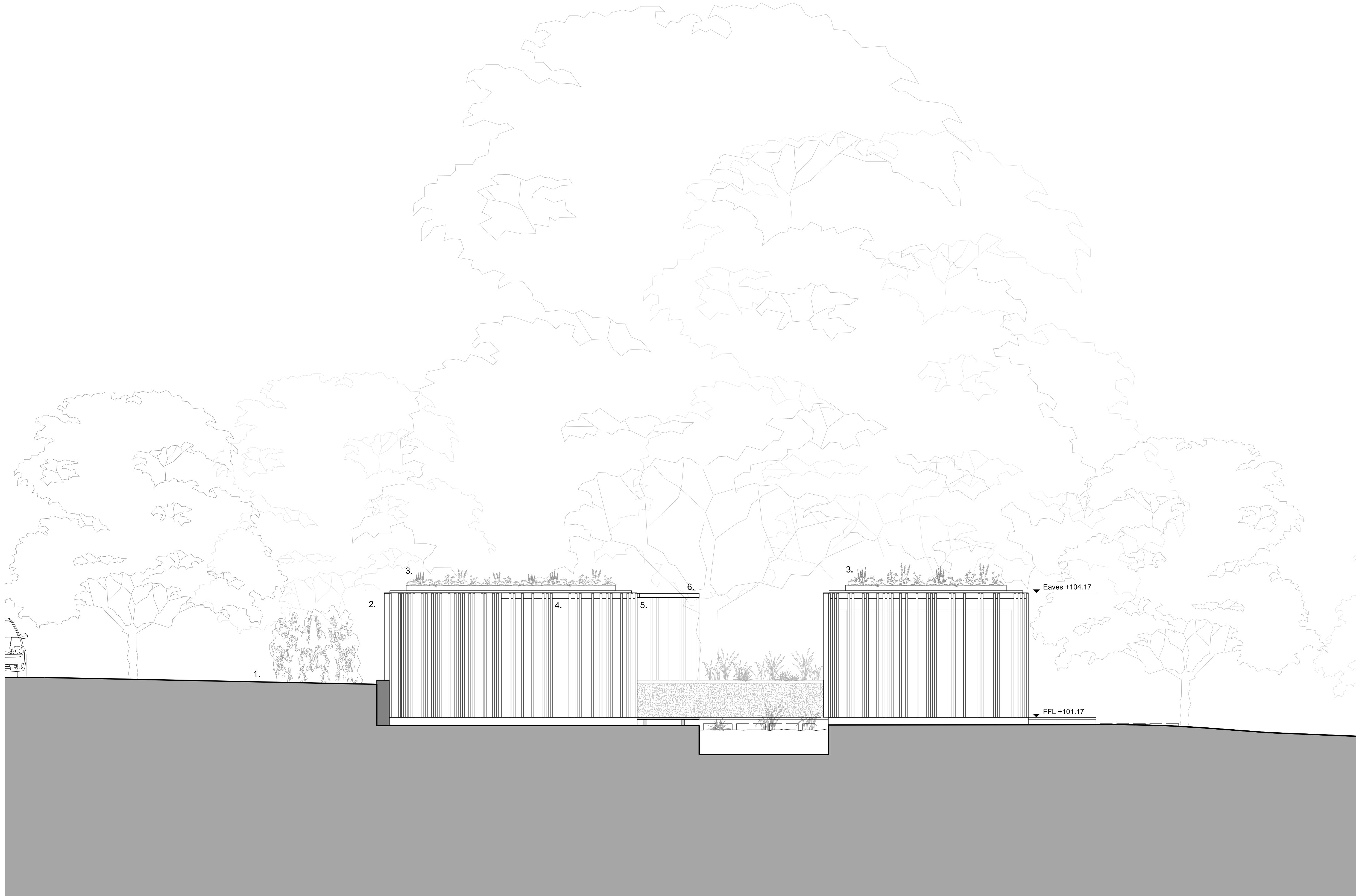
01 Proposed Pool House: North-West elevation 1:50 @ A1
