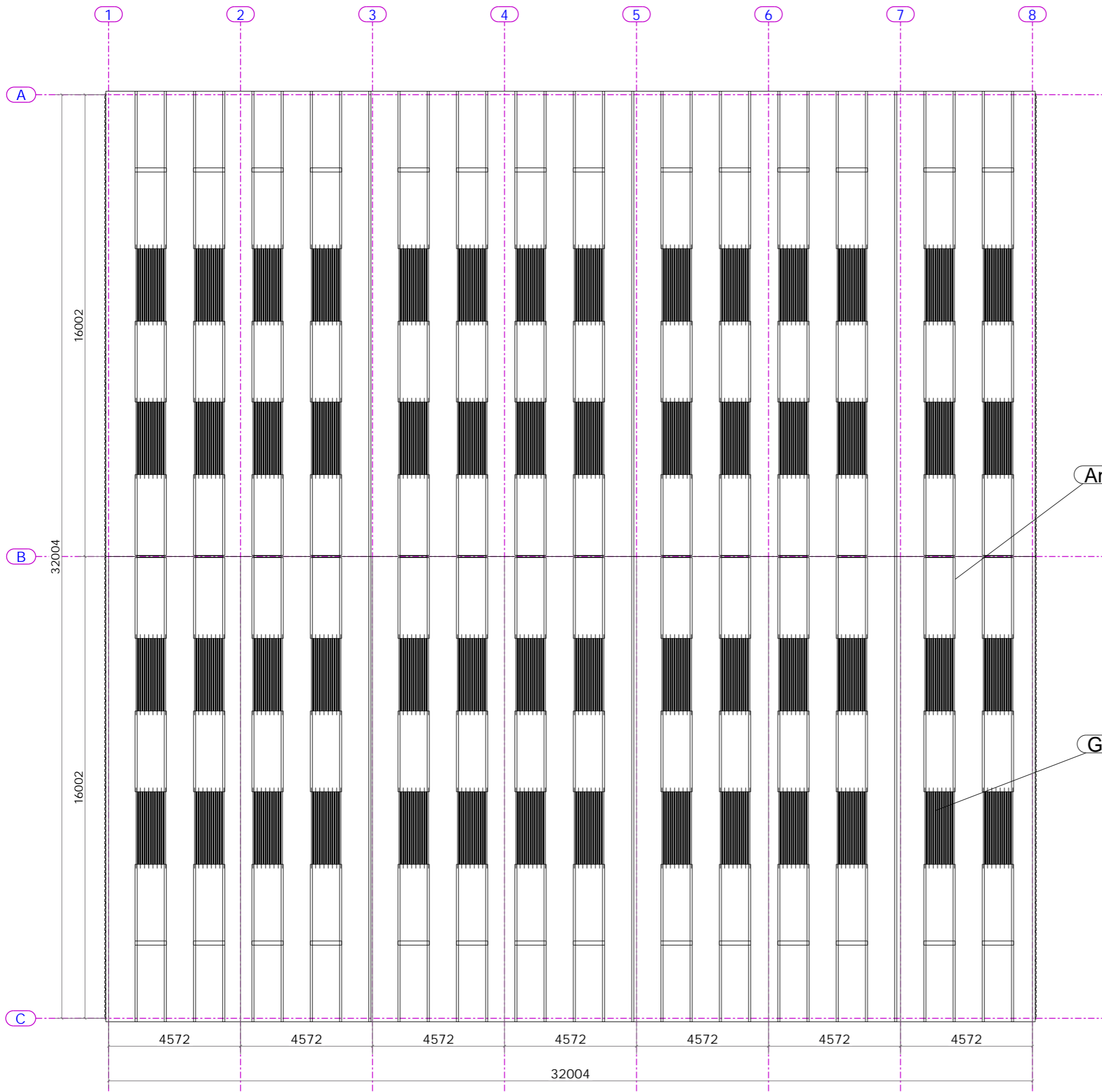
Plan EAVES
