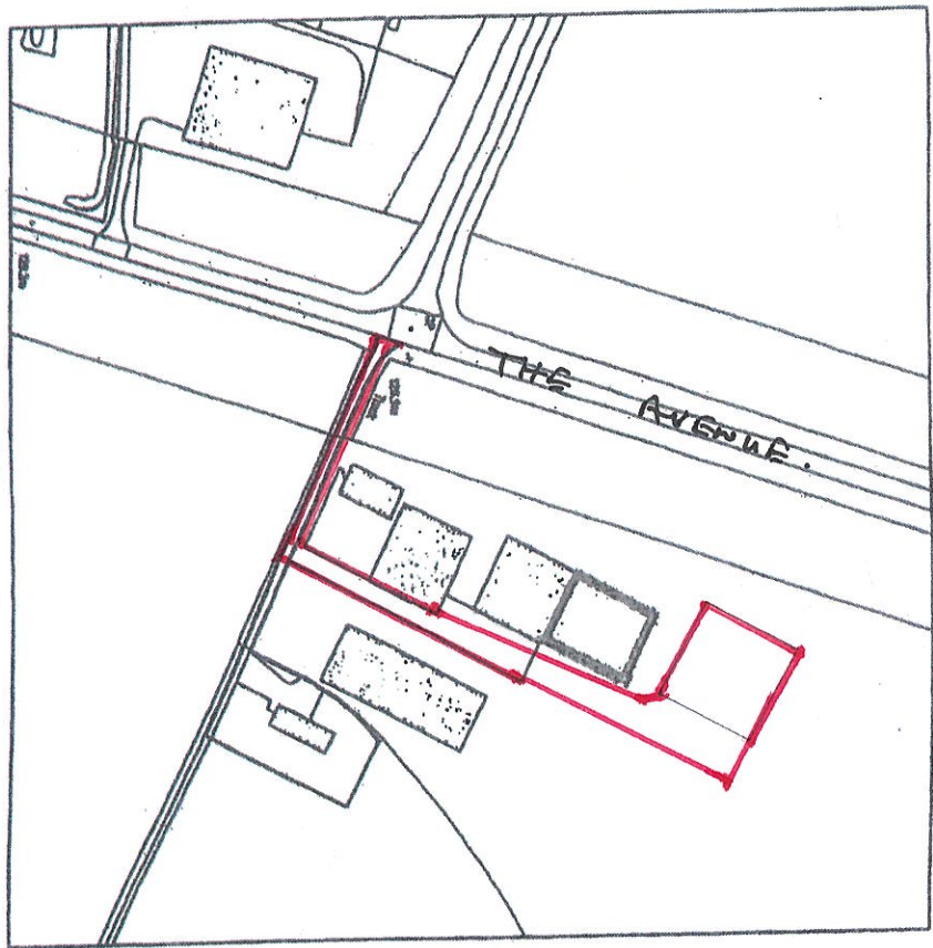
Site Plan + Location Plans Scale - 1:1250 @ A3
