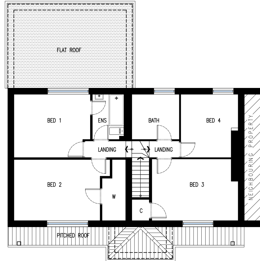
[02] EXISTING FIRST FLOOR PLAN 1:100
