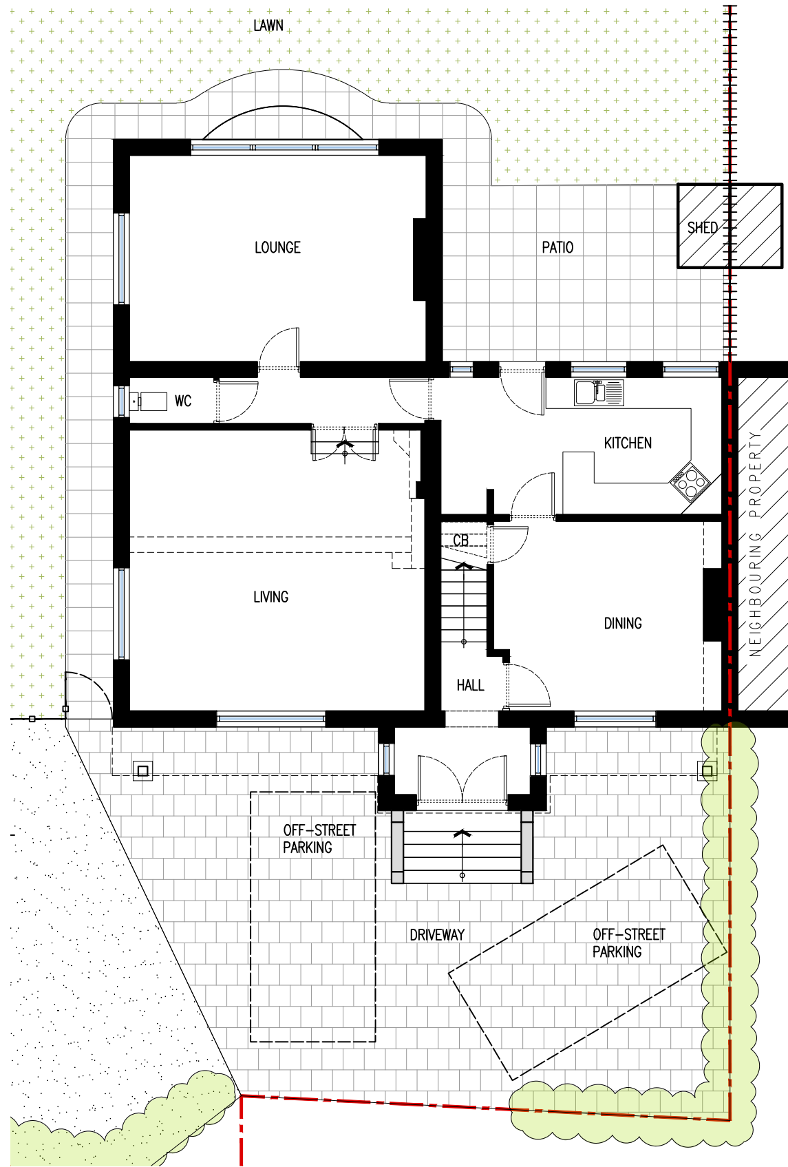
[01] EXISTING GROUND FLOOR PLAN 1:100
