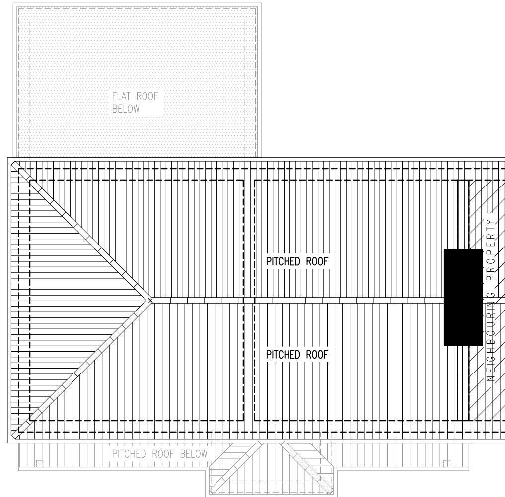
[01] EXISTING / PROPOSED ROOF PLAN 1:100
