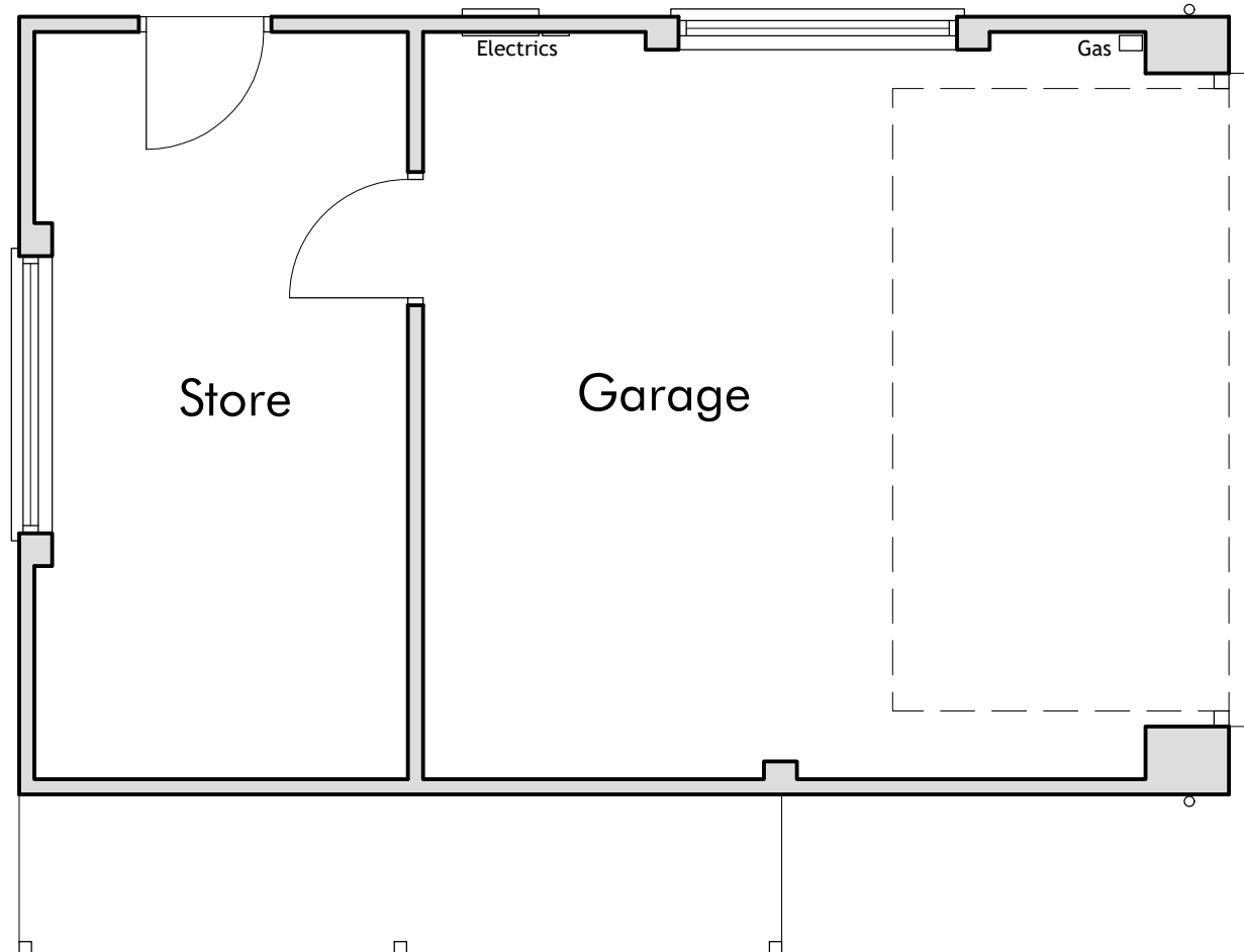
Floor Plan (1:50)
