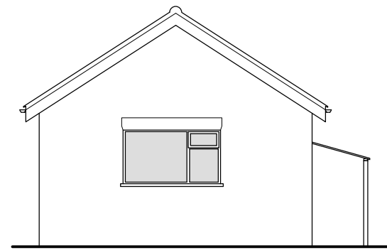
West Elevation (1:100)
