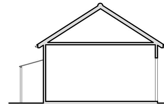
Typical Section (1:100)
