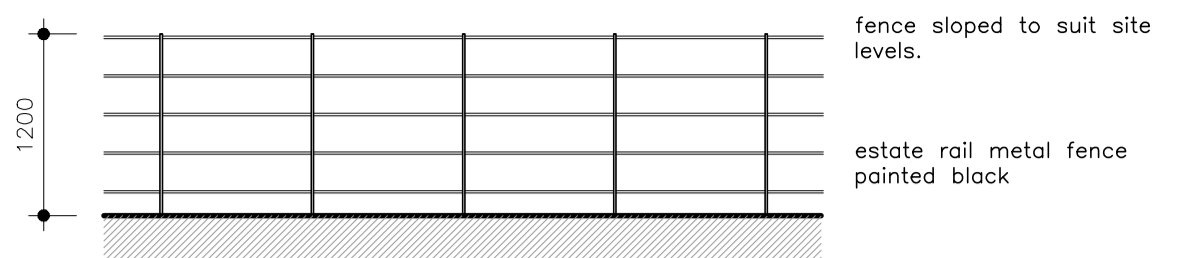
FENCE TYPE A PROPOSED scale 1:50
