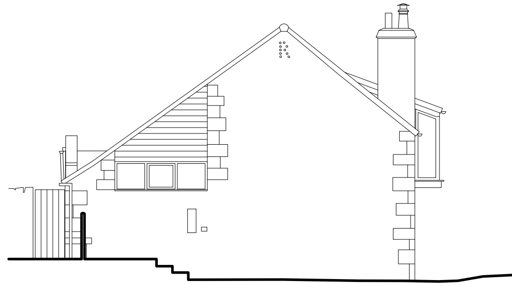
Existing Side (East) Elevation
