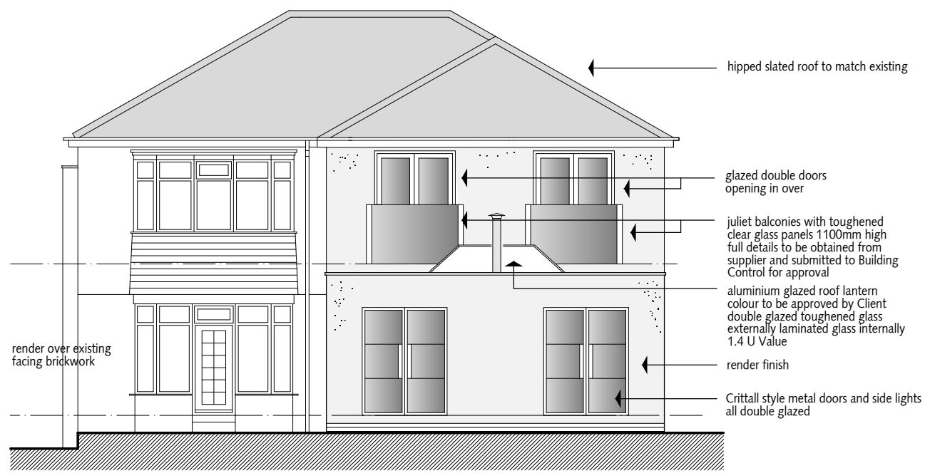
rear elevation as proposed
