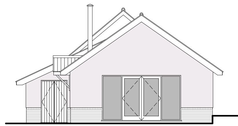
EAST ELEVATIONS 1:100.
