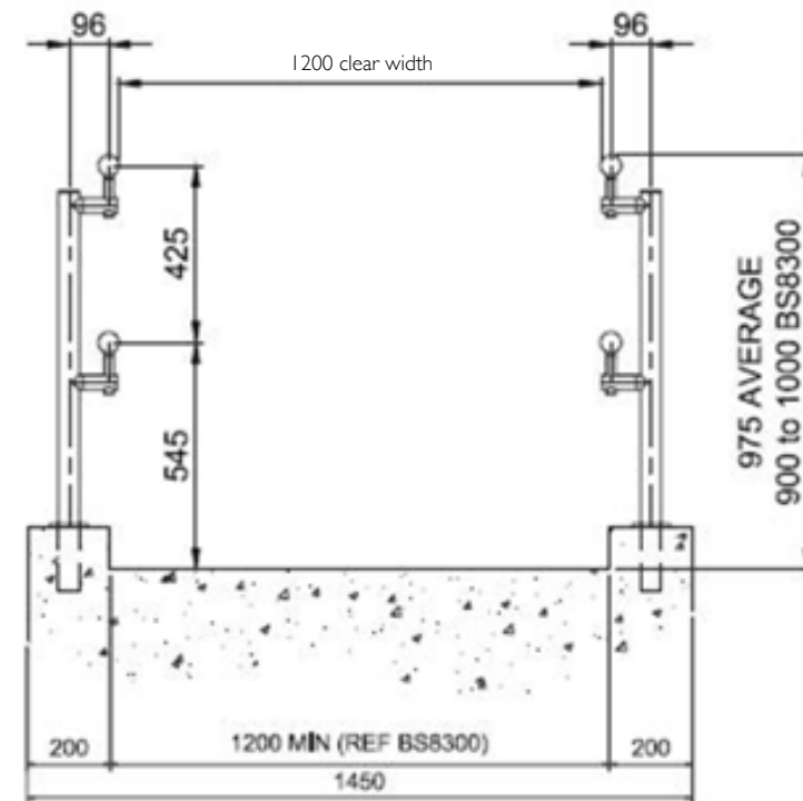
Hand Rail Detail 1:20
