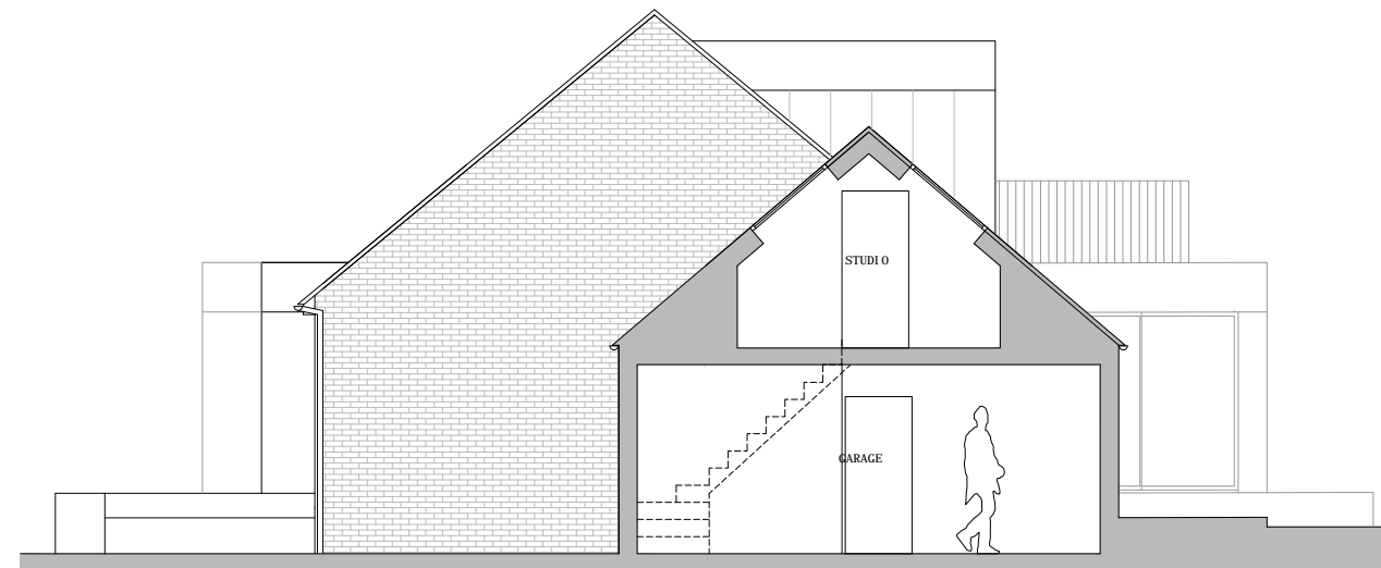
Proposed Section CC
