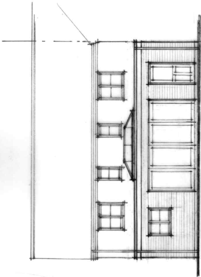
rear elevation
