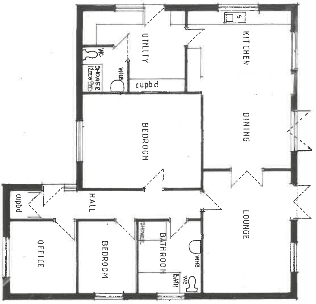
prop. floor layout
