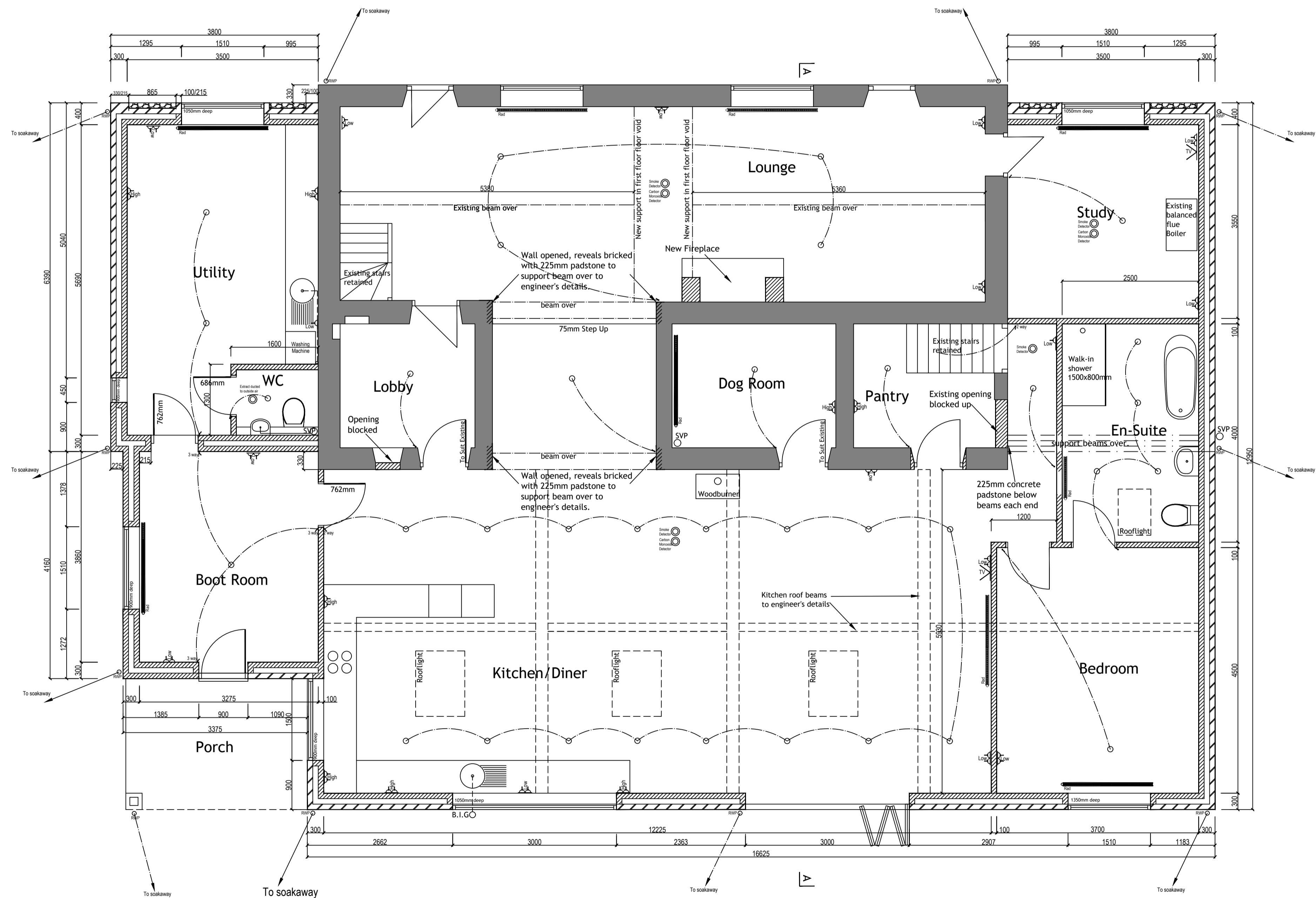
Proposed Ground Floor Layout
