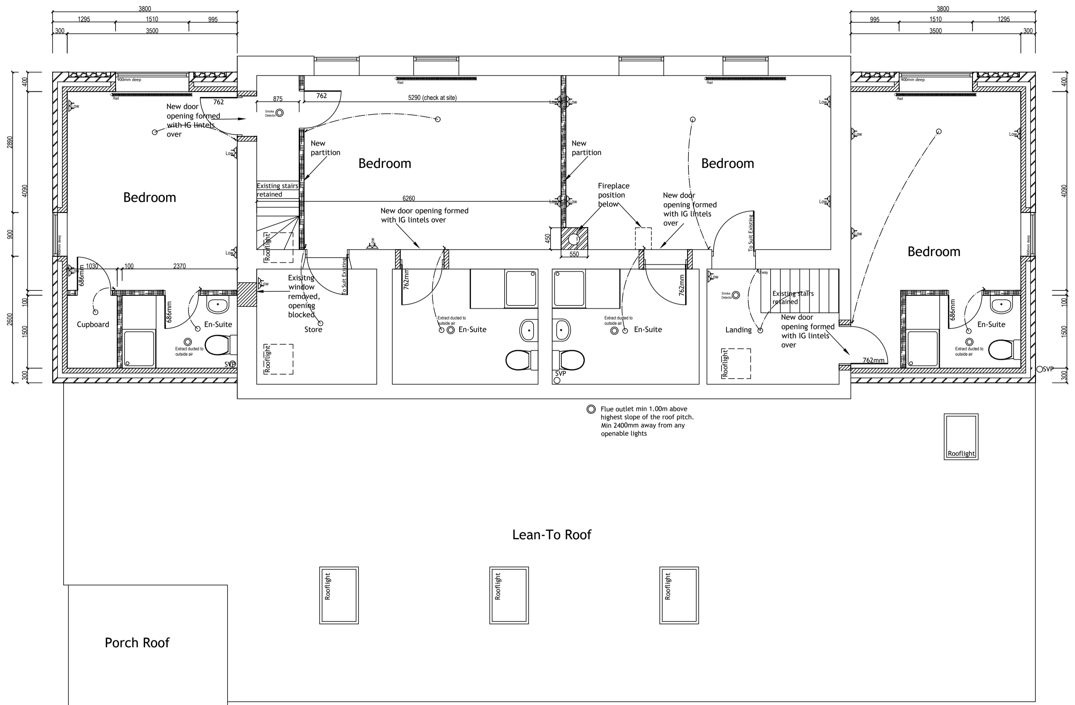
Proposed First Floor Layout
